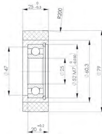
Roller: \phi 79 x 25 art. no. 141 867.09
